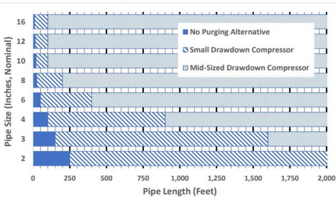
Figure 4232-3. Alternative Purging Selection: System pressures greater than or equal to 50# but less than 100#
